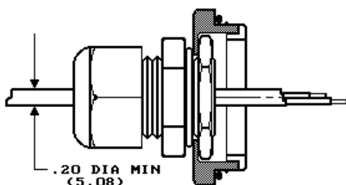
CONNECTOR INSTALLED ON RECEPTACLE CAP
